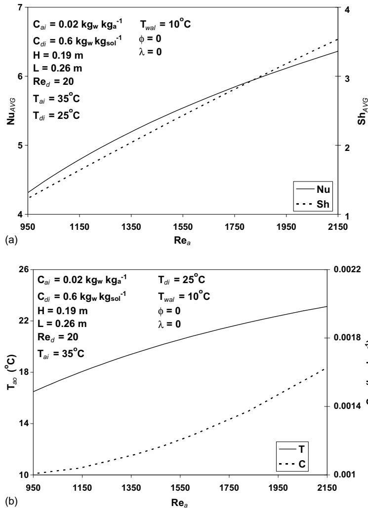
Fig. 2. Effect of air Reynolds number on dehumidification and cooling of the air on (a) Nusselt and Sherwood numbers and (b) exit air conditions.
