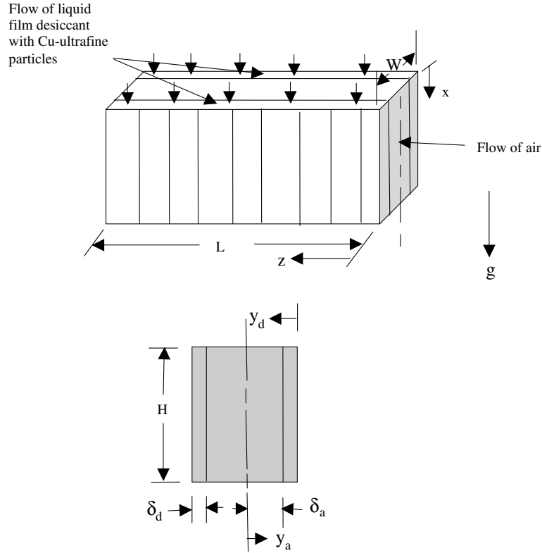
Fig. 1. Schematic of cross flow channel between air and solution.
