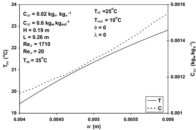
Fig. 6. Effect of channel width on dehumidification and cooling of the air on exit air conditions.
