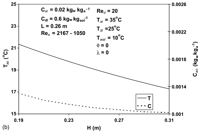
Fig. 4. Effect of channel height on dehumidification and cooling of the air on (a) average Nusselt and Sherwood numbers and (b) exit air conditions.
