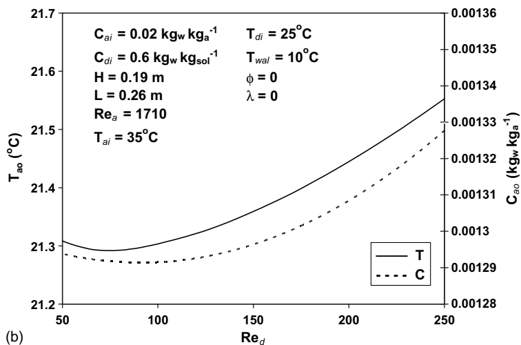
Fig. 3. Effect of solution Reynolds number on dehumidification and cooling of air on (a) average Nusselt and Sherwood numbers and (b) exit air conditions.
