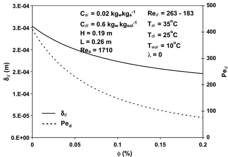
Fig. 9. Effect of partial volume fraction of Cu-ultrafine particles on solution thickness and effective Peclet number.
