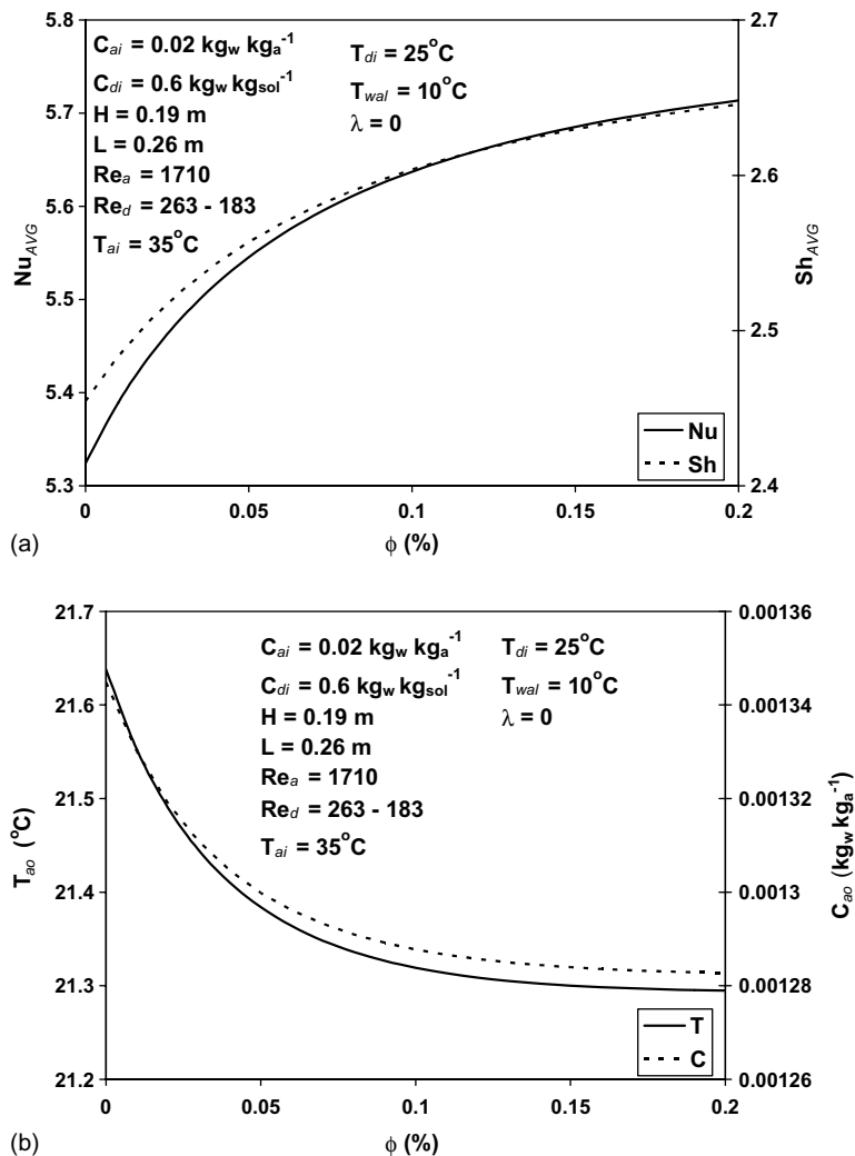
Fig. 8. Effect of volume fraction of Cu-ultrafine particles on dehumidification and cooling of the air on (a) average Nusselt and Sherwood numbers and (b) exit air conditions.
