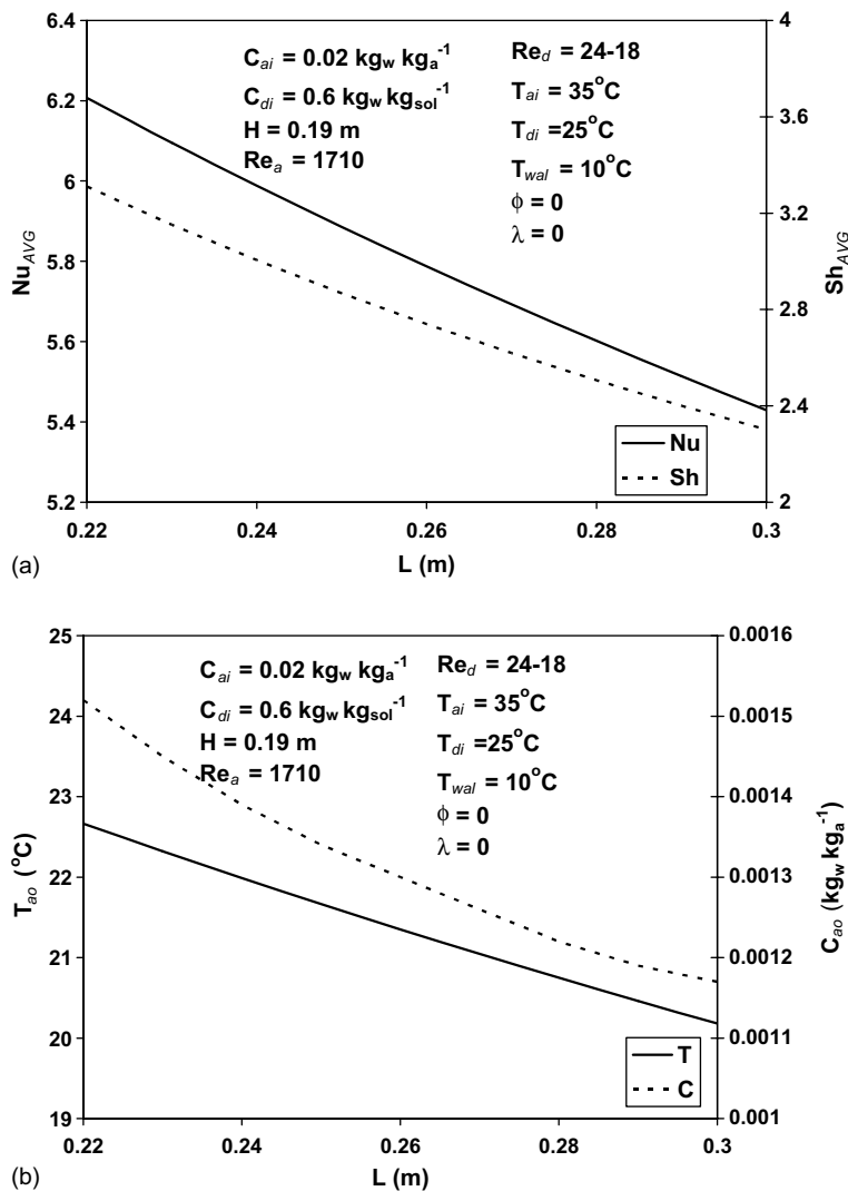
Fig. 5. Effect of channel length on dehumidification and cooling of the air on (a) average Nusselt and Sherwood numbers and (b) exit air conditions.
