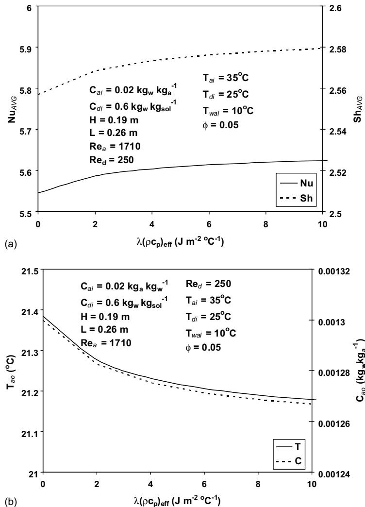
Fig. 10. Effect of dispersion factor of Cu-nanoparticle suspensions for dehumidification and cooling of the air on (a) average Nusselt and Sherwood numbers and (b) exit air conditions.
